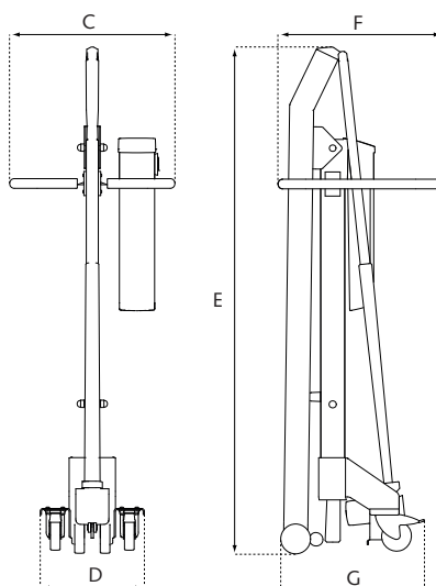
Dimensions (mm)
